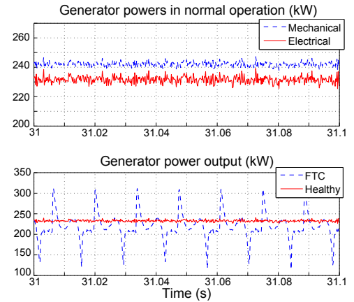
Figure 7. Generator input power and output power for healthy and faulty conditions.
