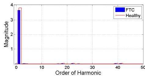
Figure 10. Harmonics spectrum of grid currents for healthy and faulty generator conditions.
