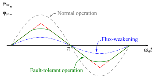
Figure 4. Stator flux waveforms for healthy and faulty machine.
