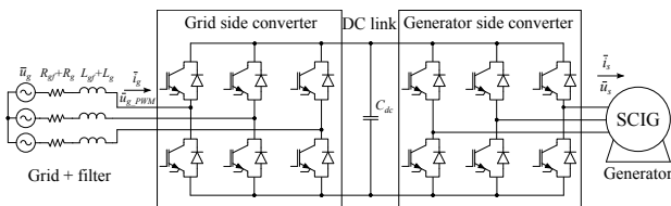
Figure 1. Back to back power converter topology in wind turbines.
