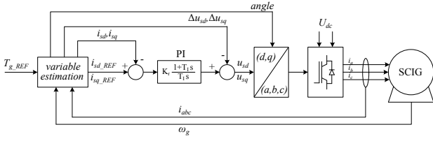
Figure 2. Field-oriented control loop.
