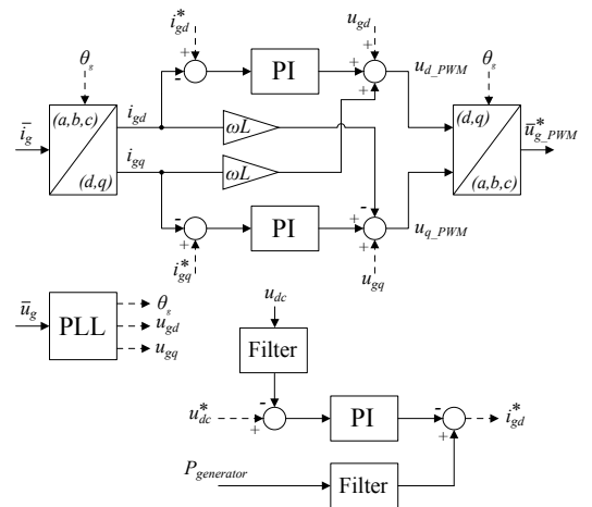
Figure 3. Basic voltage-oriented control loop.
