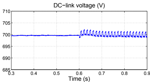
Figure 8. DC-link voltage for healthy and faulty generator conditions.
