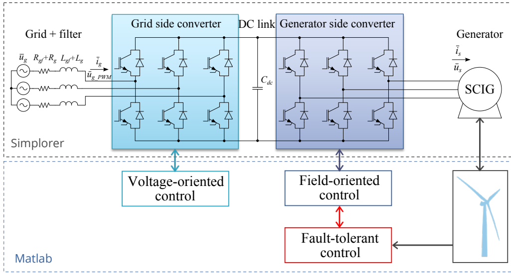
Figure 6. Simulation scheme with denoted Simplerer and Matlab part.
