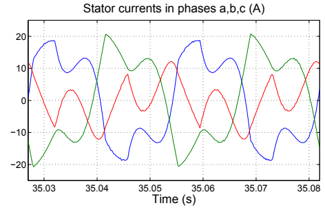
Figure 5. Generator stator currents with applied fault-tolerant control.
